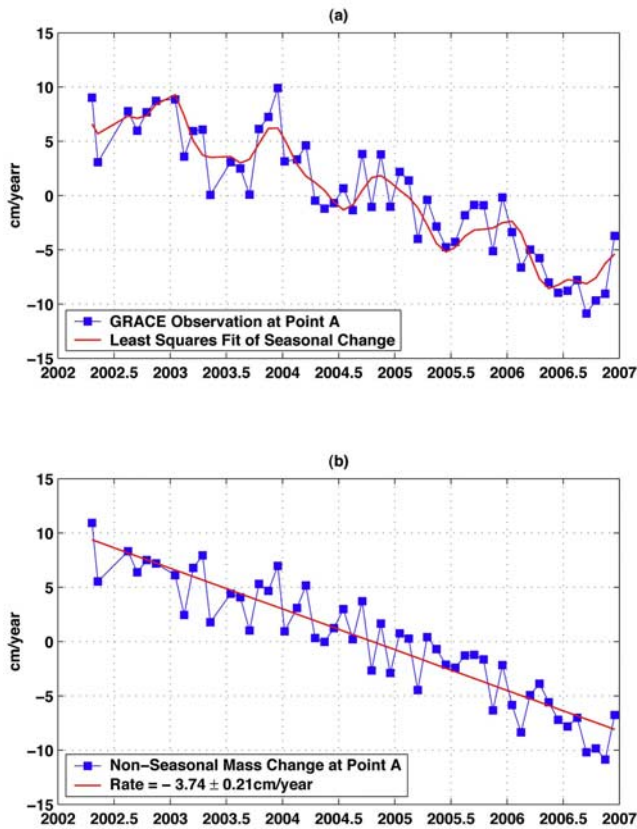
Figure 3. (a) GRACE mass changes (in blue curve with square markers) from the 53 RL04 gravity solutions at location A, marked in Figure 1. The red curve represents the least square fit of a linear trend, seasonal (annual and semiannual) sinusoids, and a 161-day tidal aliasing term. (b) Non-seasonal mass change (in blue curve with square markers) from GRACE at the same location. The red line is the linear trend from the least squares fit.
