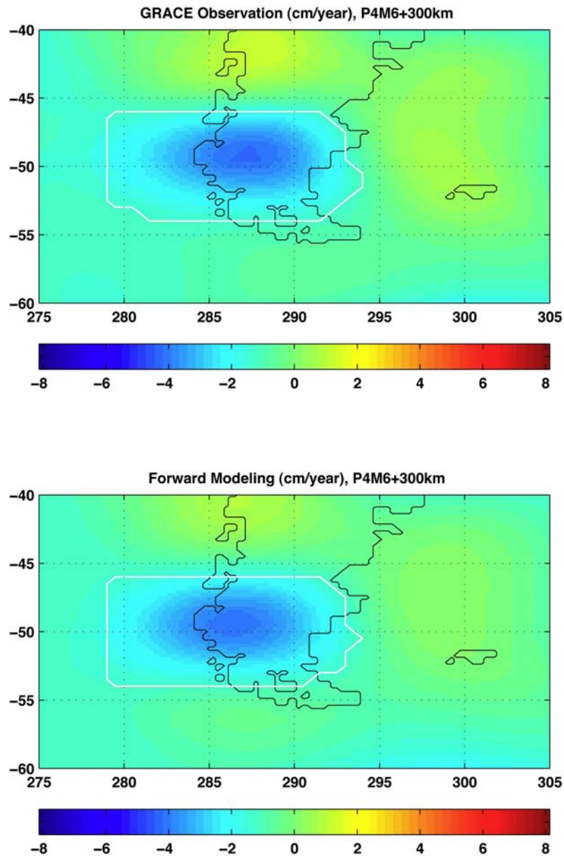
Figure 5. (top) Same GRACE observations (as in Figure 2) interpolated onto 0.25^\circ \times 0.25^\circ grids (from the original 1^\circ \times 1^\circ grid). The white lines circle the area within which rate magnitude drops below 1 cm/year, defining the anomaly region. (bottom) Forward modeling rate map prediction (also 0.25^\circ \times 0.25^\circ grids). The white lines circle the area where the rate magnitude drops below 1 cm/yr. The areas circled by white boxes are the regions in which we sum total mass rate with cosine of latitude weighting, as described in the text.
