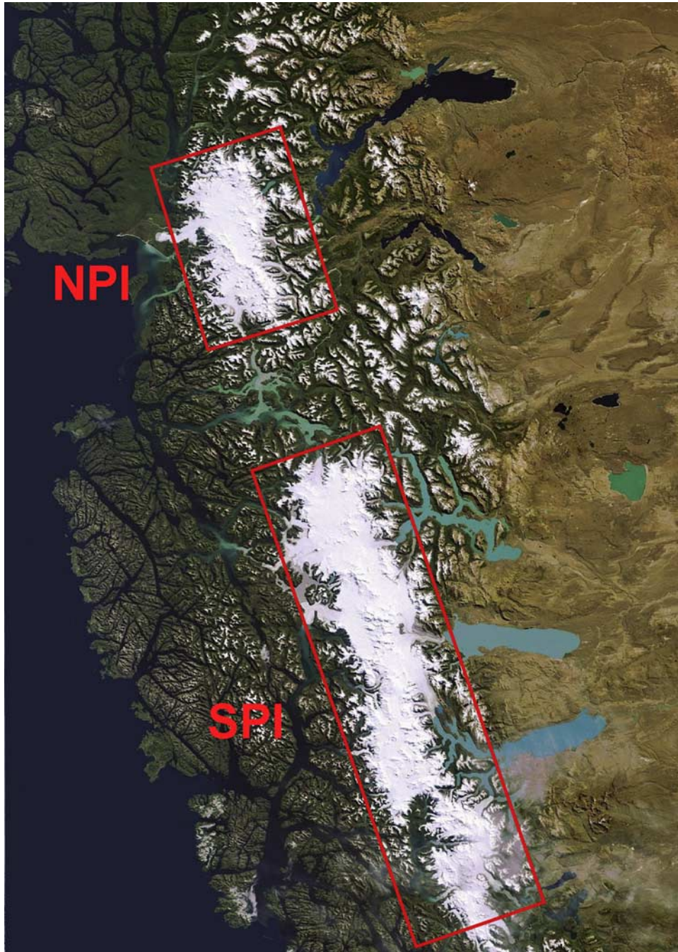
Figure 1. A satellite image of the Northern Patagonia Icefield (NPI) and Southern Patagonia Icefield (SPI) in South America, as circled by the red boxes. The original image is provided by the European Space Agency.
