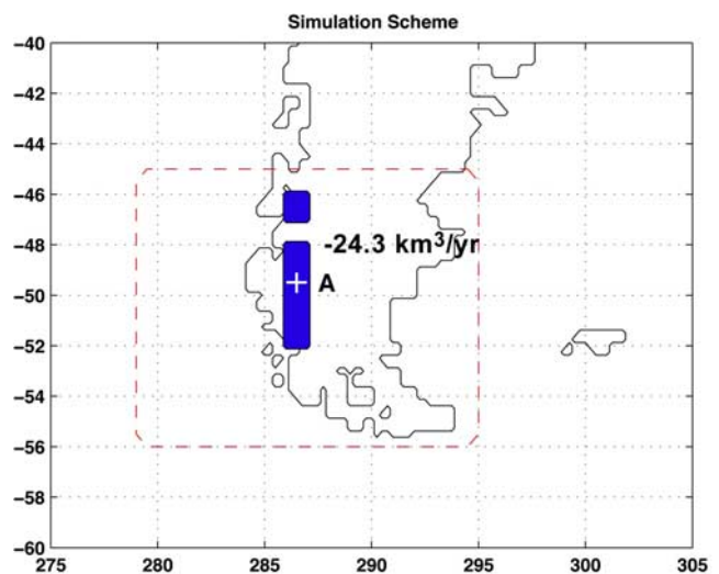
Figure 4. Illustration of the forward modeling scheme: The two shaded areas represent the NPI and SPI areas, respectively. A total mass rate of \sim -24.3 \text{ km}^3/\text{year} is uniformly distributed over the two shaded areas. Mass changes at grid points outside the red box are adopted from GRACE observation (as shown in Figure 2). The white cross marks point (A) for which time series are shown in Figure 3.
