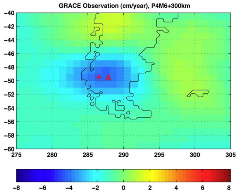
Figure 2. GRACE linear mass rates (in units of cm of equivalent water height change per year, cm/yr) for April 2002 to December 2006, in the PIF region. The 2-step filtering involves application of a decorrelation filter to remove noise stripes at certain SH orders, followed by 300 km Gaussian smoothing. Mass rates are estimated from the 53 time series values at each grid point using least squares to fit the linear trend, seasonal, and tidal alias sinusoids.
